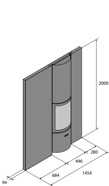
Stûv 30-in frontpaneel
